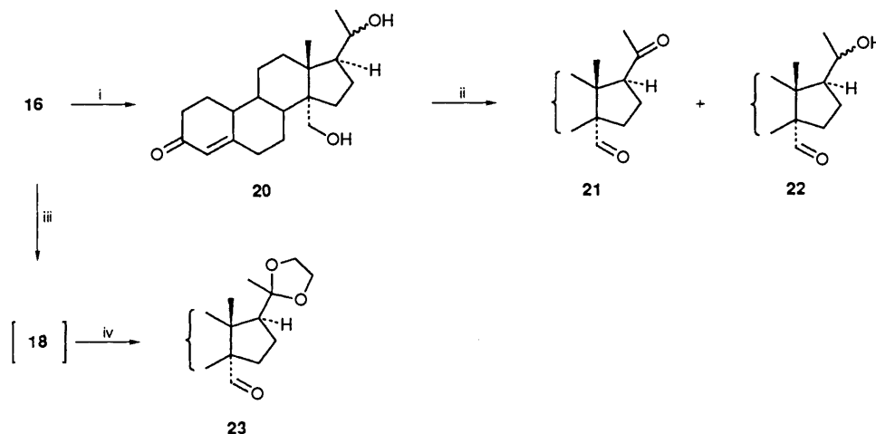
Scheme 4 Reagents and conditions: i, Li-NH 3 - tert -BuOH; ii, C 5 H 5 + NHCrO 3 Cl - , 0 °C; iii, (CH 2 OH) 2 - p TsOH, heat; iv, (C 5 H 5 N + H) 2 C 2 O 7 2- , 25 °C
