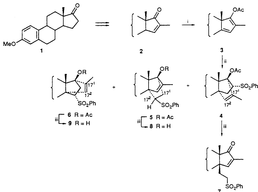
Scheme 1 Reagents and conditions: i, \text{Ac}_2\text{O}-\text{CH}_3\text{CO}_2\text{C}(\text{CH}_3)=\text{CH}_2-p\text{TsOH} , 100^\circ\text{C} ; ii, \text{CH}_2=\text{CHSO}_2\text{Ph} , 140^\circ\text{C} ; iii, \text{KOH}-\text{MeOH} , 25^\circ\text{C}
