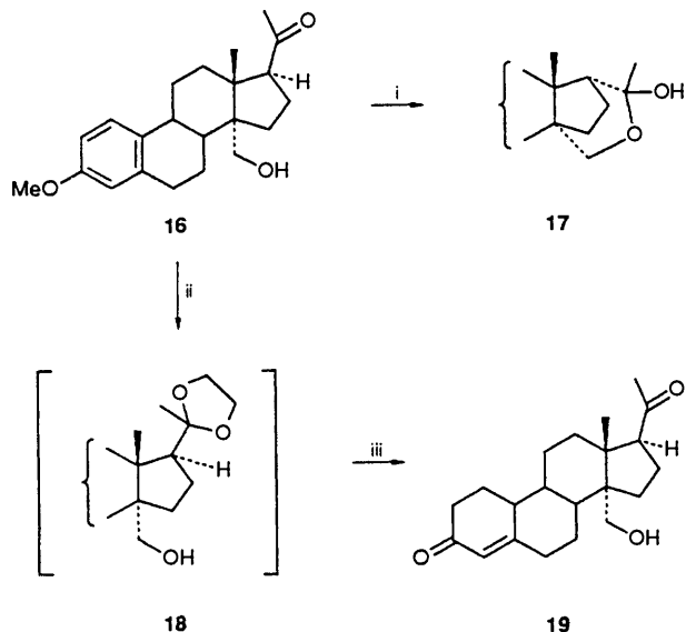
Scheme 3 Reagents and conditions: i, KOH-MeOH, 60 °C; ii, (CH 2 OH) 2 - p TsOH, heat; iii, Li-NH 3 - tert -BuOH, then HCl-MeOH
