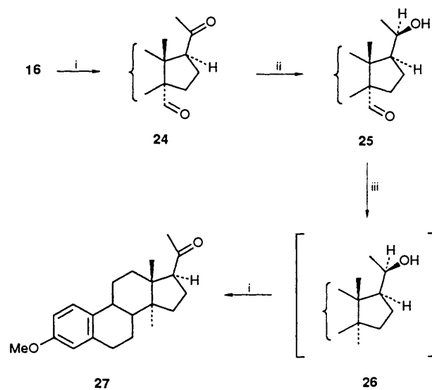
Scheme 5 Reagents and conditions: i, C 5 H 5 + NHCrO 3 Cl - , 0 °C; ii, LiBu 3 BH, 0 °C; iii, N 2 H 4 -KOH, 215 °C
